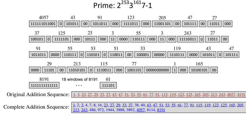
Fig. 2. Hybrid windowing method for 2^a \ell_B^b f - 1
