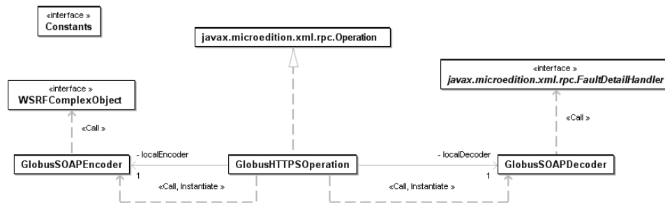
Figure 2 WSRF-ME Framework Runtime
